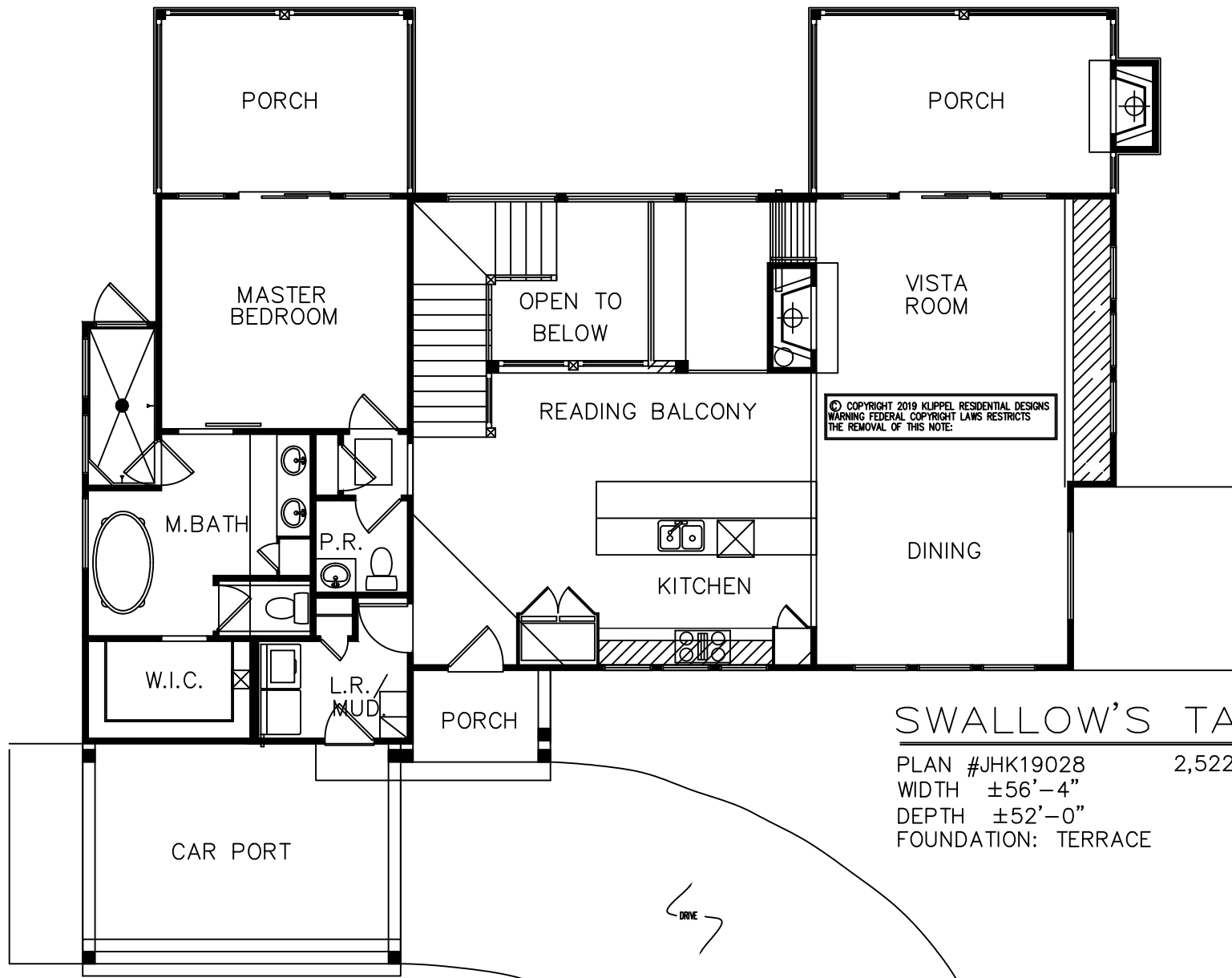
1st FLOOR PLAN 1,449 SQ. FT. CARPORT 176 SQ. FT.
